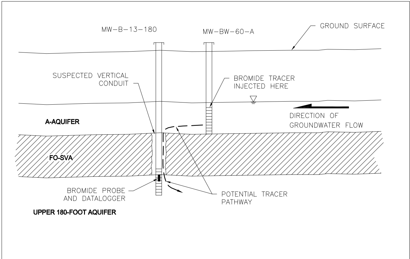
CROSS SECTION NOT TO SCALE
