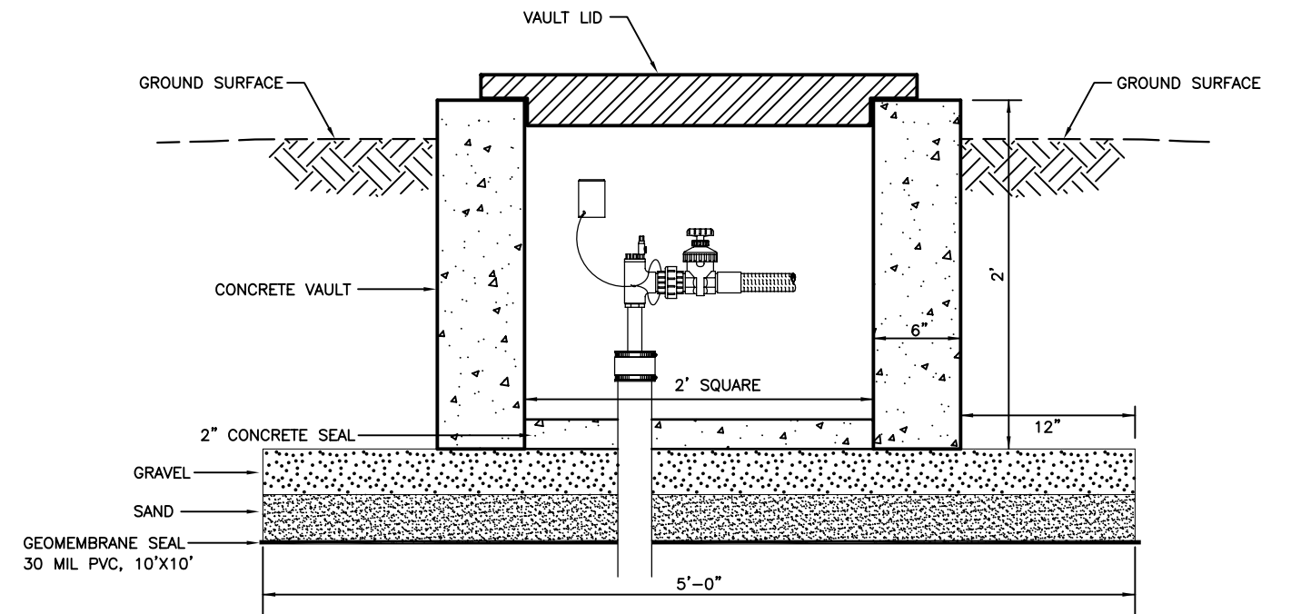
WELL VAULT DETAIL ① NOT TO SCALE
