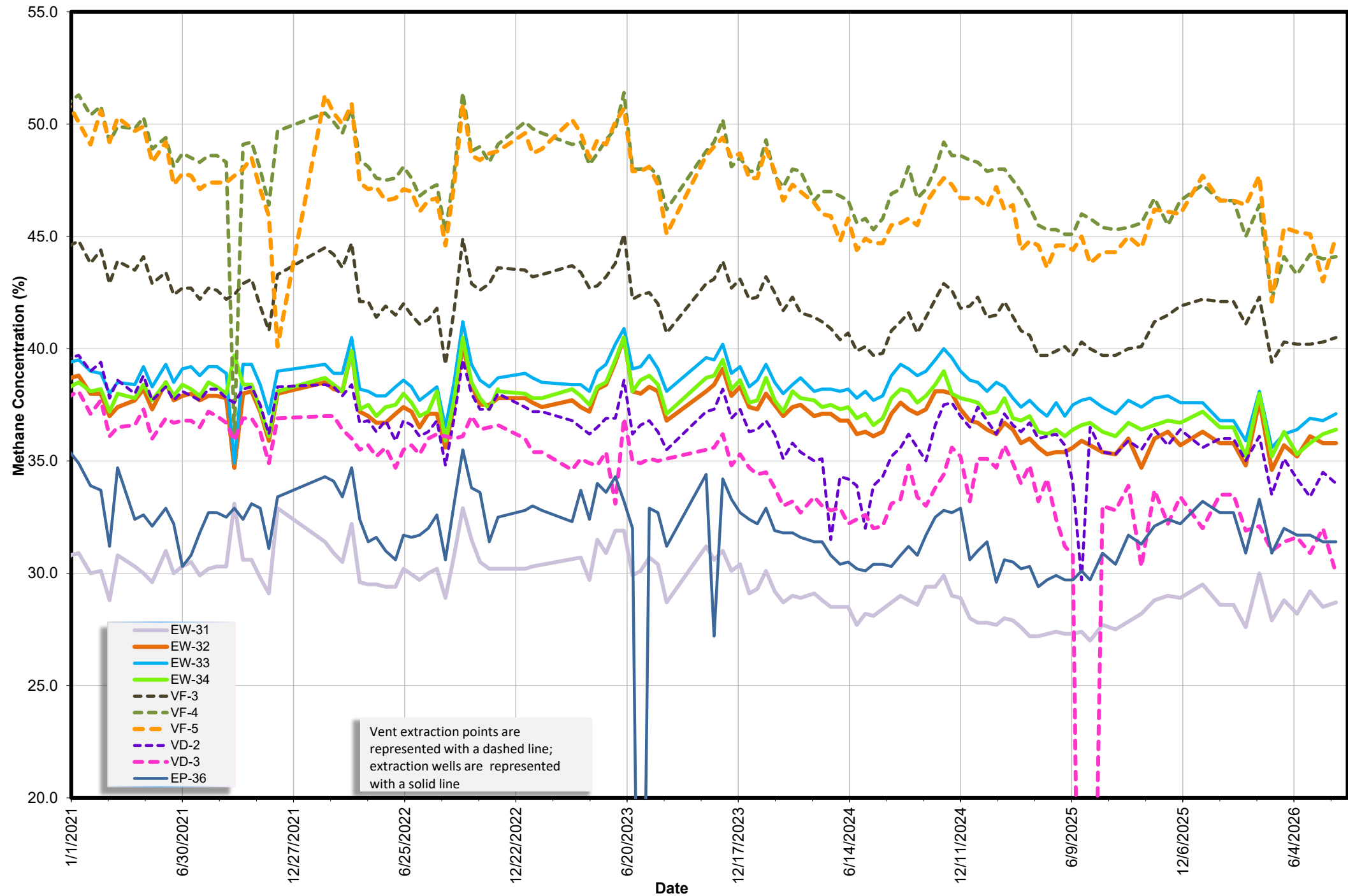
Methane Concentration Time Series Plot OU2 Landfill Individual Extraction Sources 1/2021 to present
