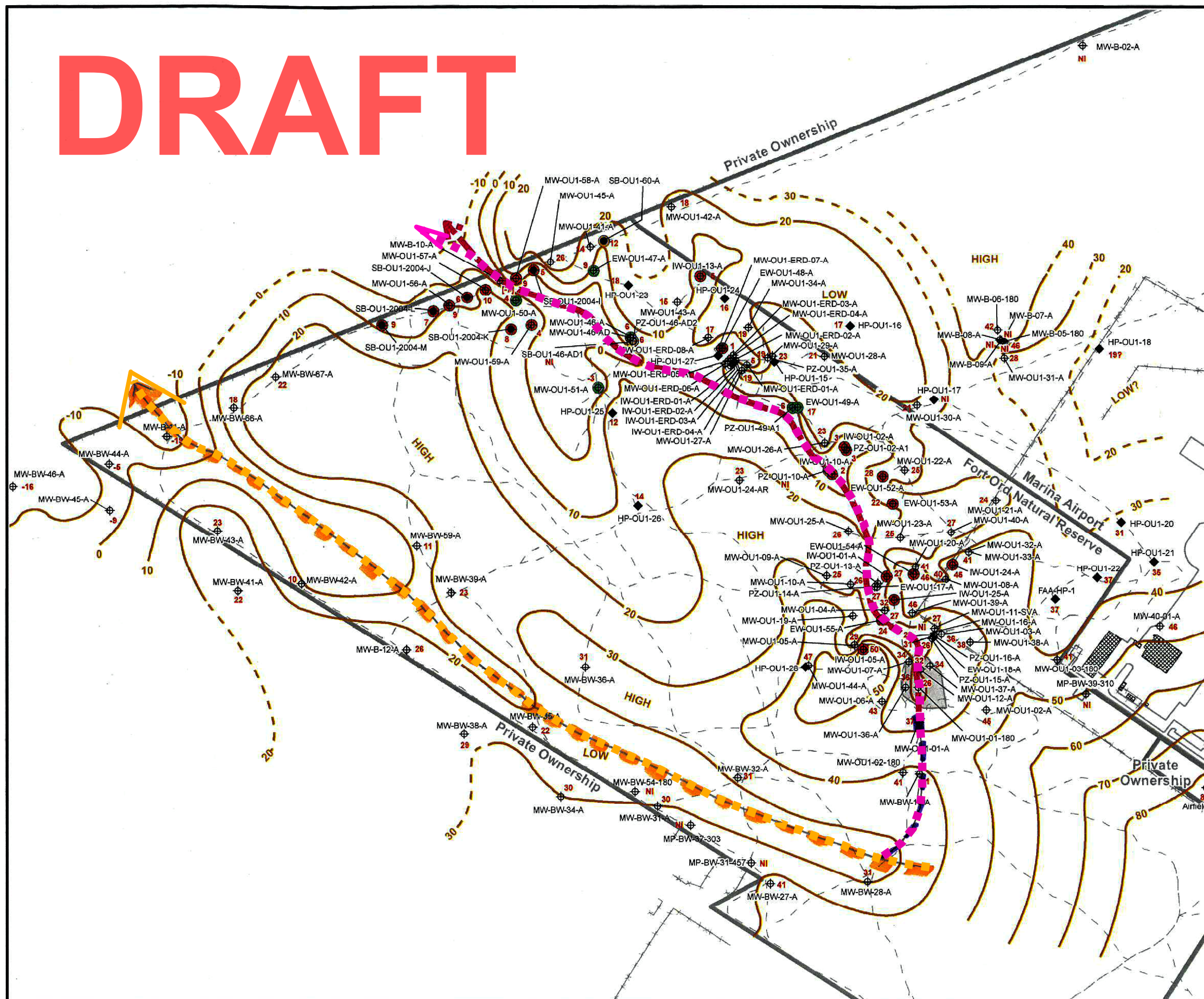
Figure 4.4A Salinas Valley Aquiclude (SVA) Elevation Contour Map - Large View Operable Unit 1 Area Former Fort Ord, CA
