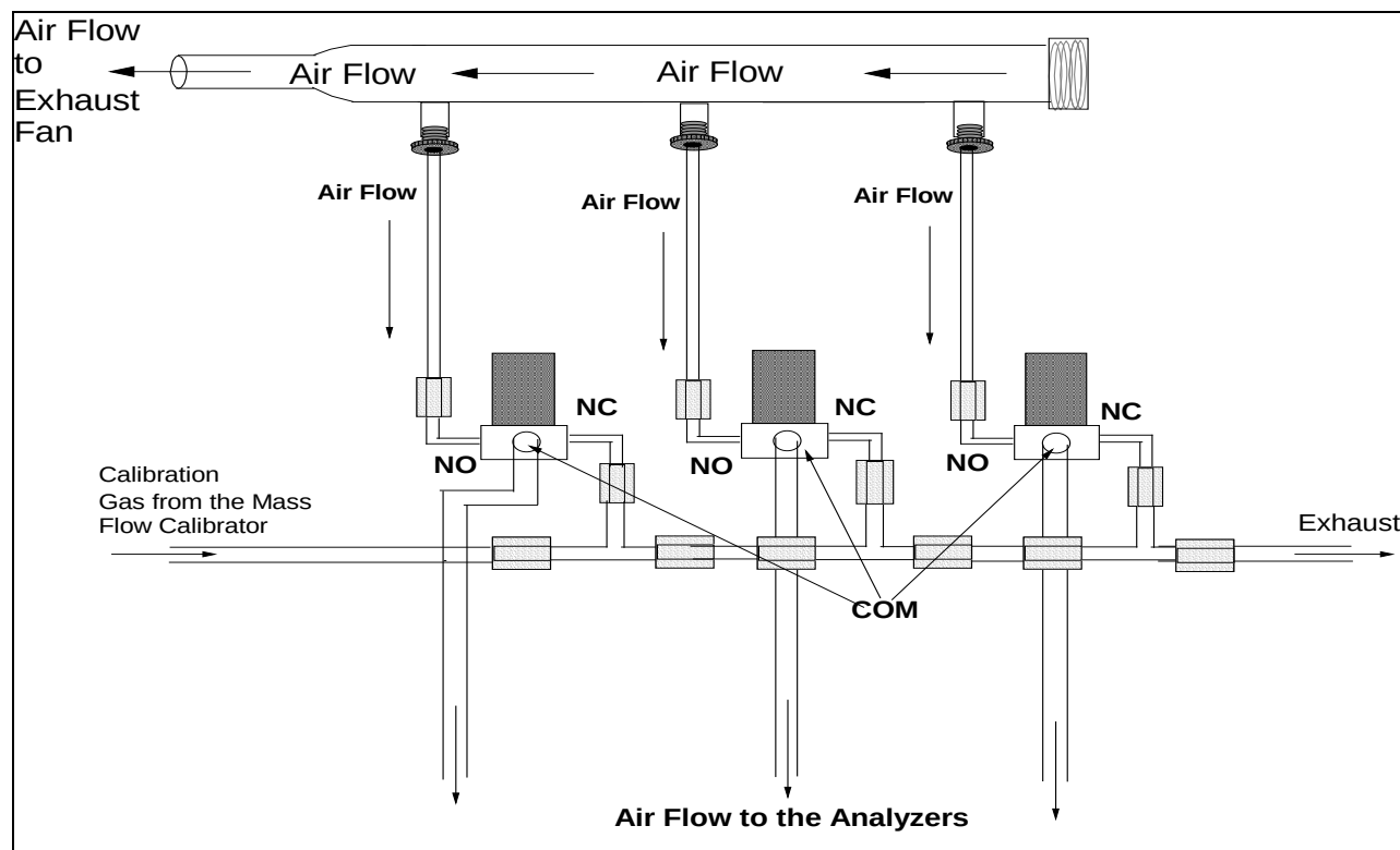
Figure 7. Ambient – Calibration Manifold Interface
