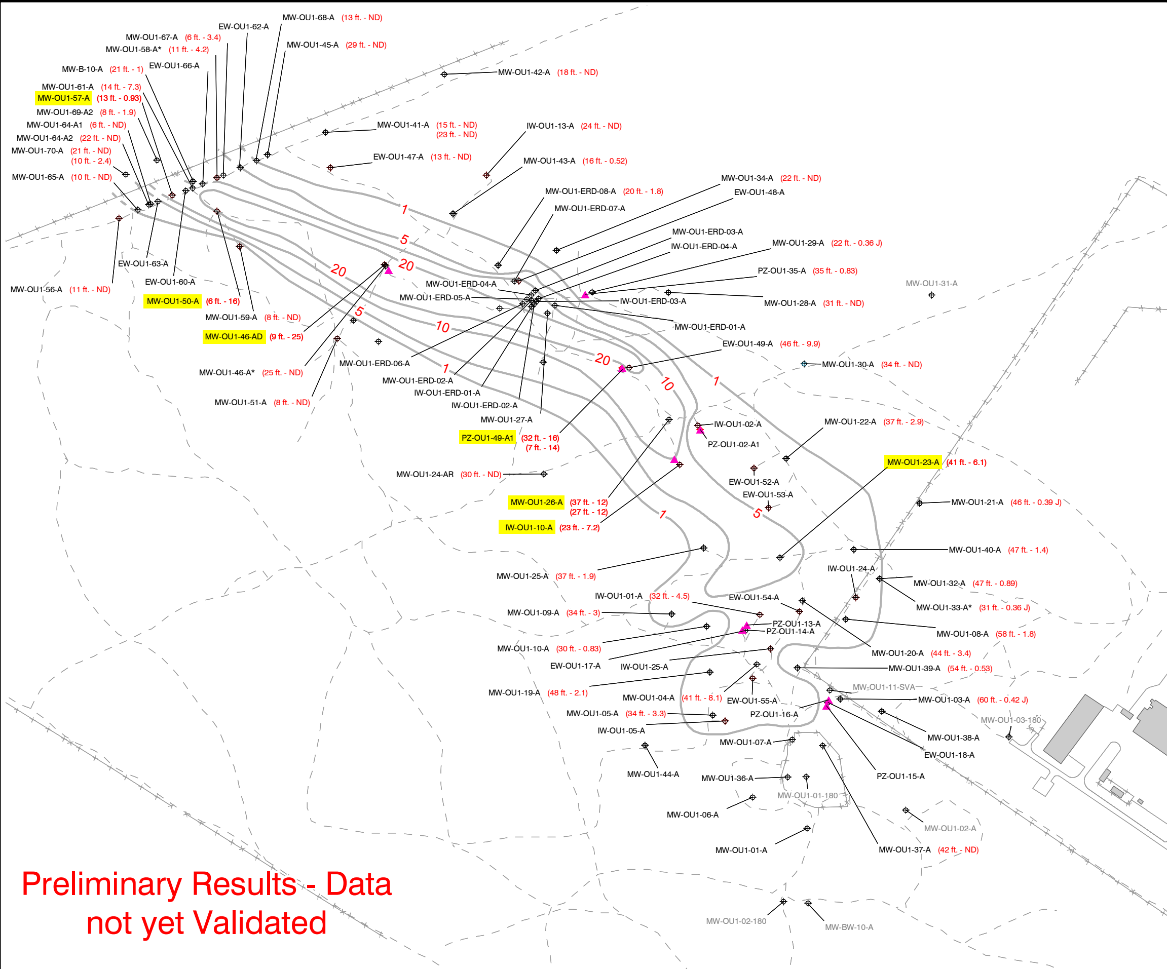
Figure 1.2 TCE Concentrations in OU-1 FONR Groundwater September 2006
